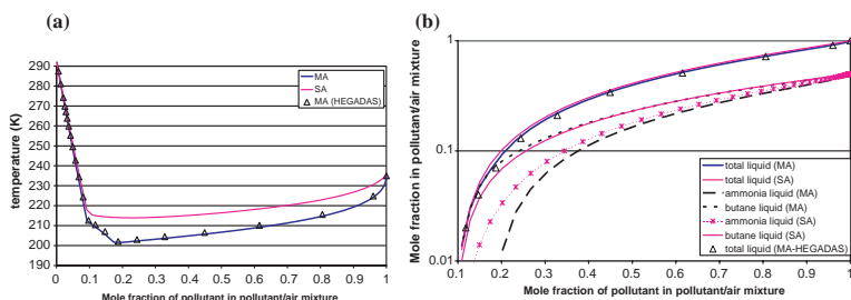
Figure 8. Mixing of ammonia/butane pollutant with dry air (MA versus SA method)
