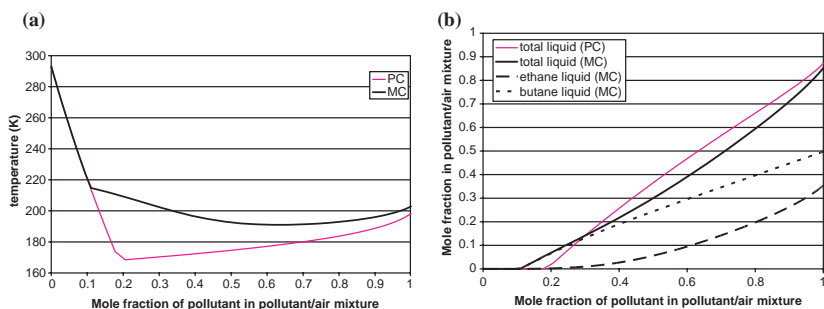
Figure 7. Mixing of ethane/butane pollutant with dry air (MC versus PC method)
